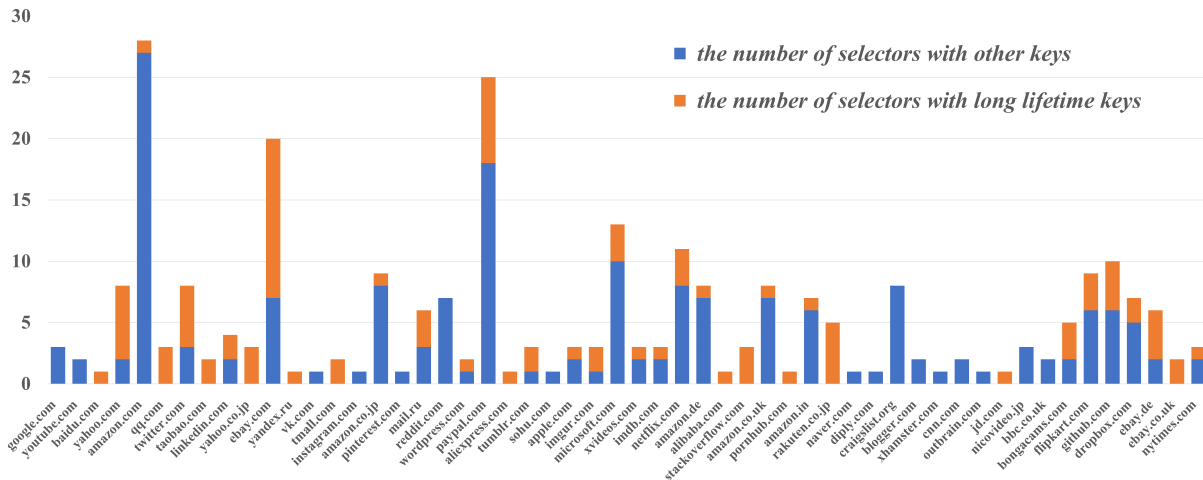
Figure 6: Selector Numbers for Popular Domains. We analyze DKIM keys lifetime of Alexa top 100 domains. The red bars represent the number of selectors, which have not changed their DKIM keys for a long time (5 years here).
